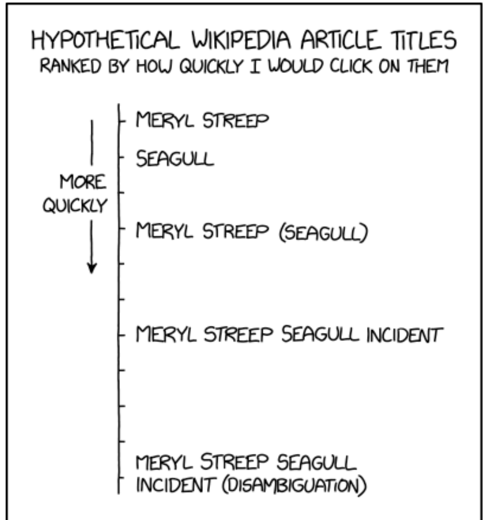
Figur 1: https://xkcd.com/2782/
